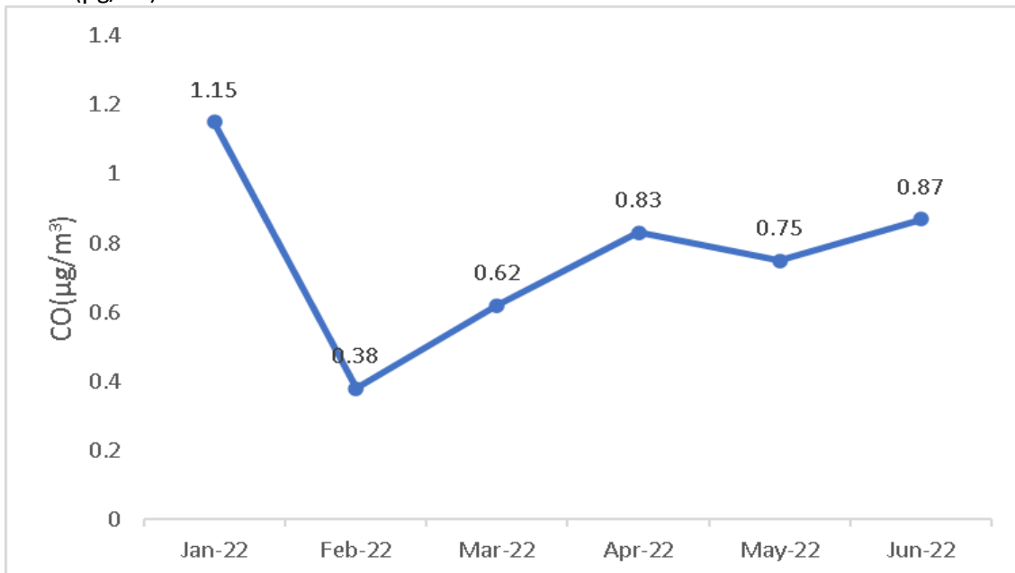
CO( \mu\text{g}/\text{m}^3 ) Line Graph
