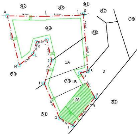
DETAILS OF BOUNDARY PILLARS
