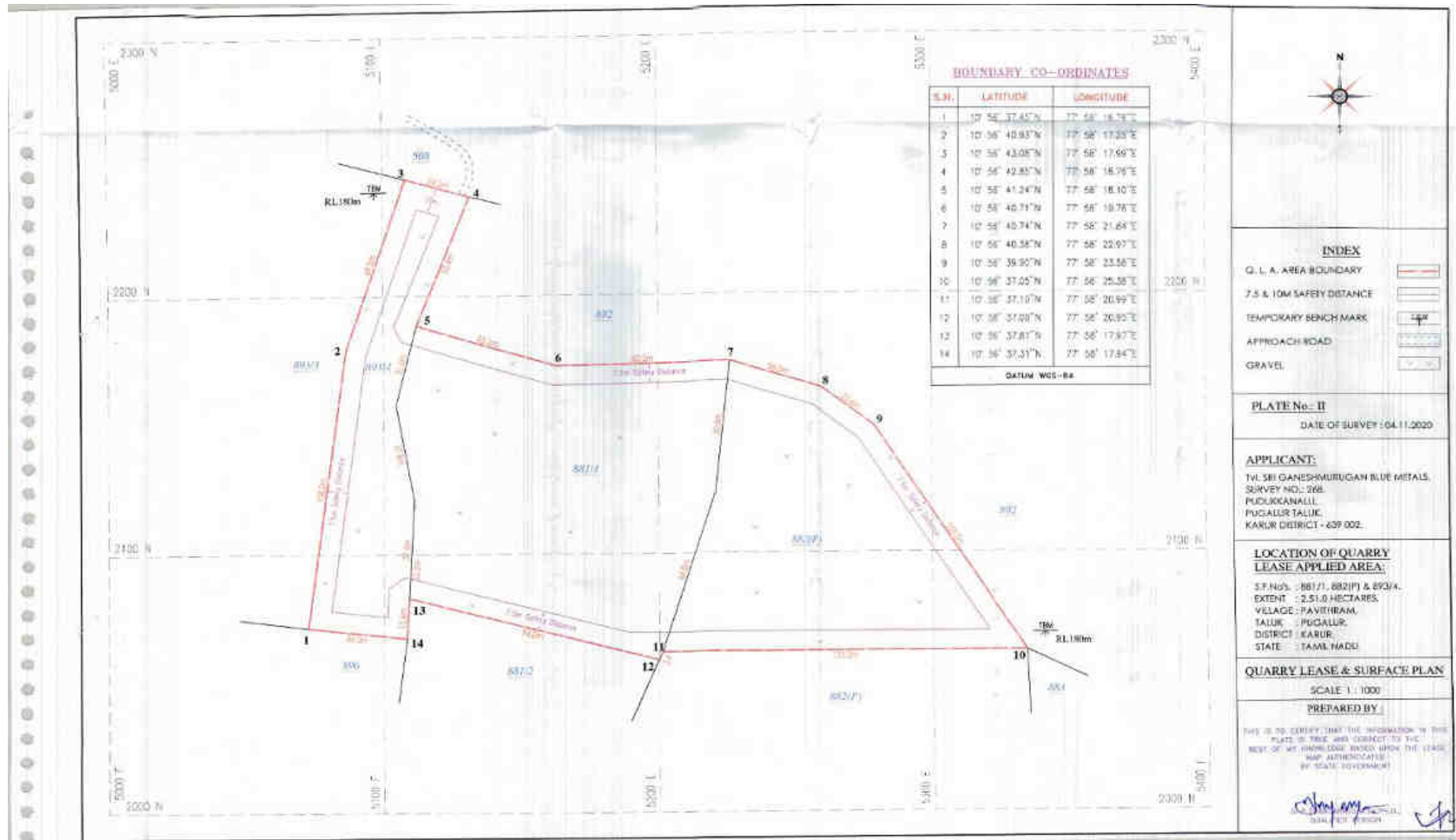
FIGURE – 4: QUARRY LEASE PLAN & SURFACE PLAN
