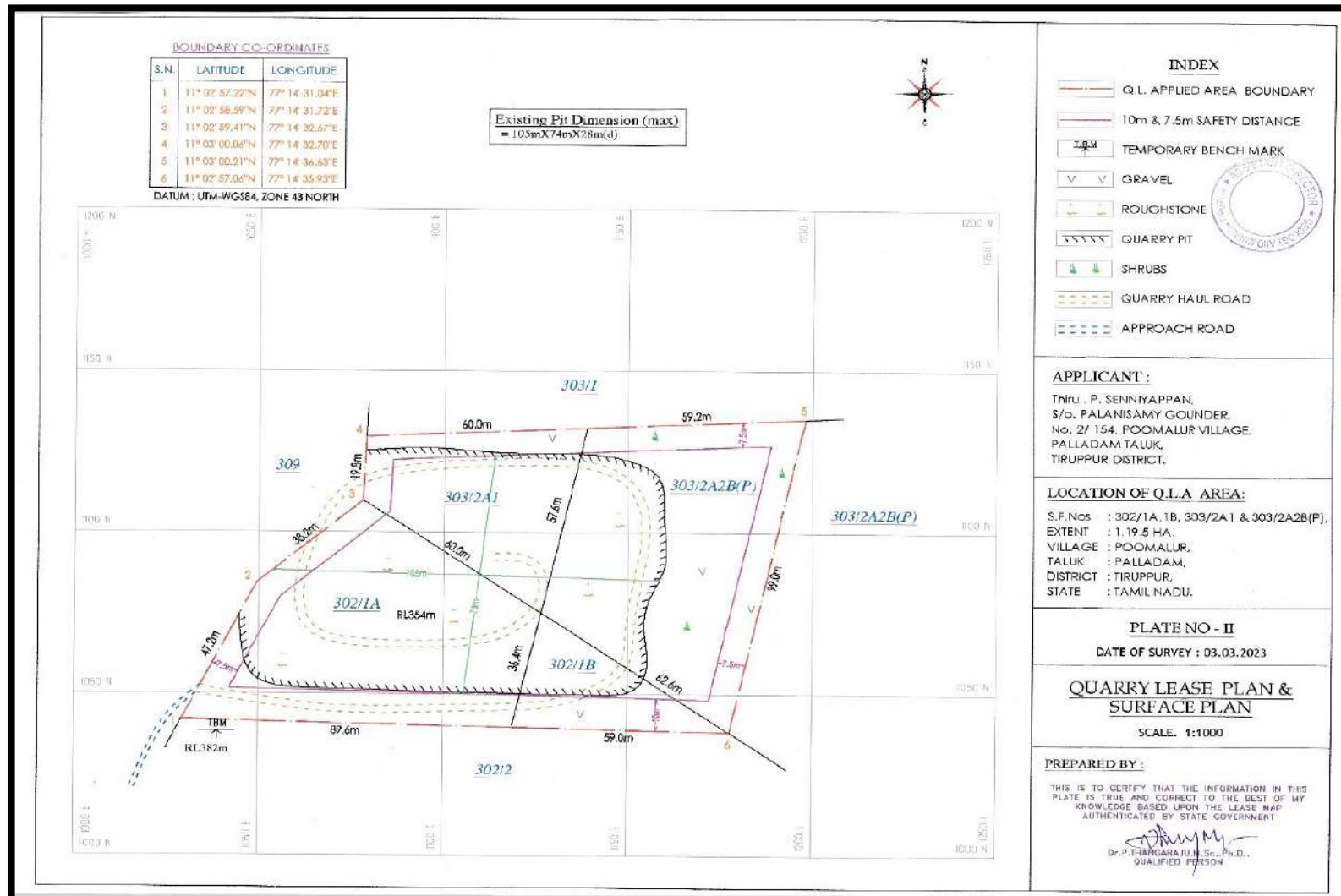
FIGURE 3: QUARRY LEASE PLAN / SURFACE PLAN
