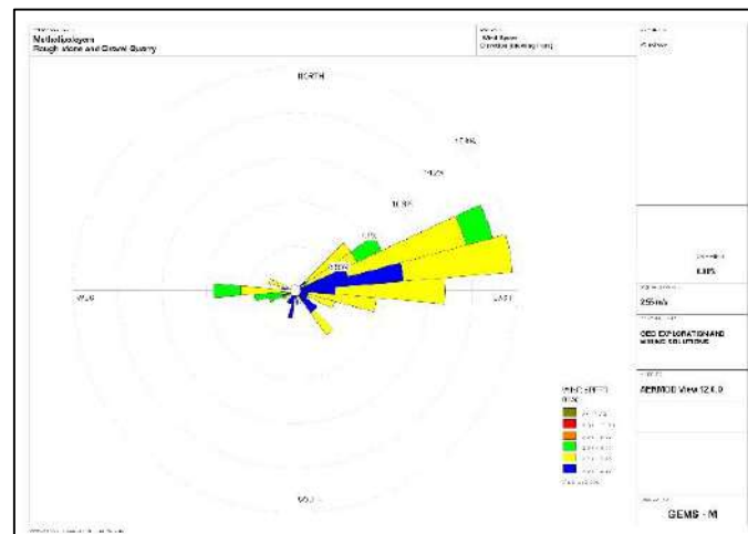
FIGURE – 5: WIND ROSE DIAGRAM
