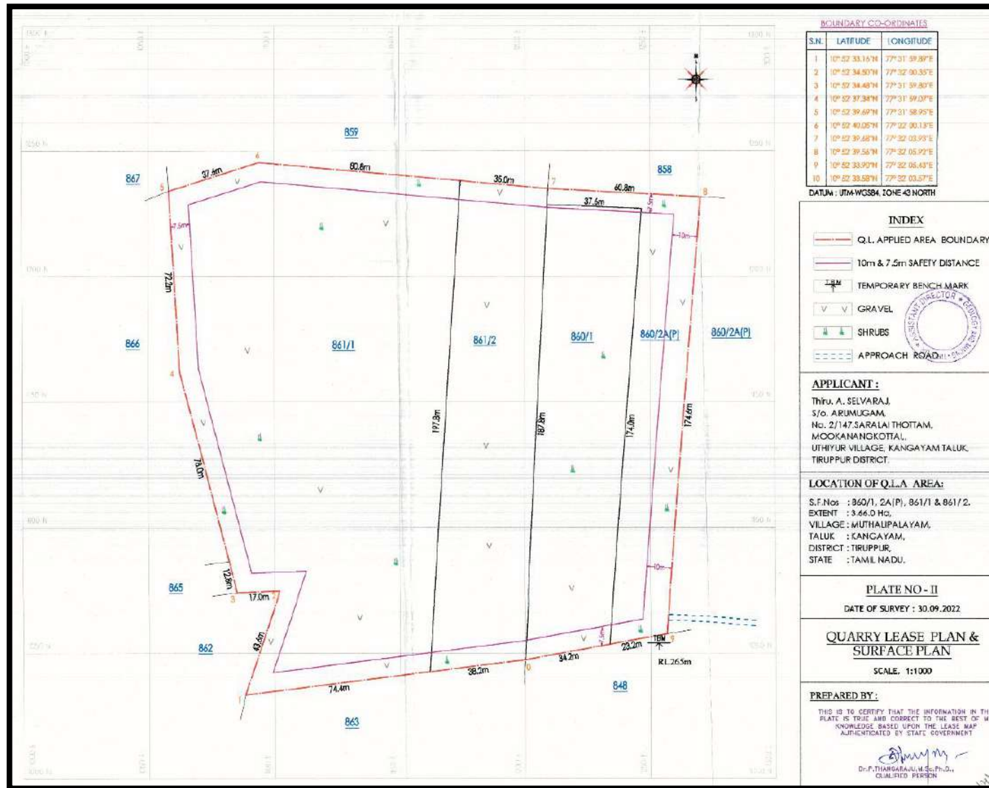
FIGURE 3: QUARRY LEASE PLAN / SURFACE PLAN
