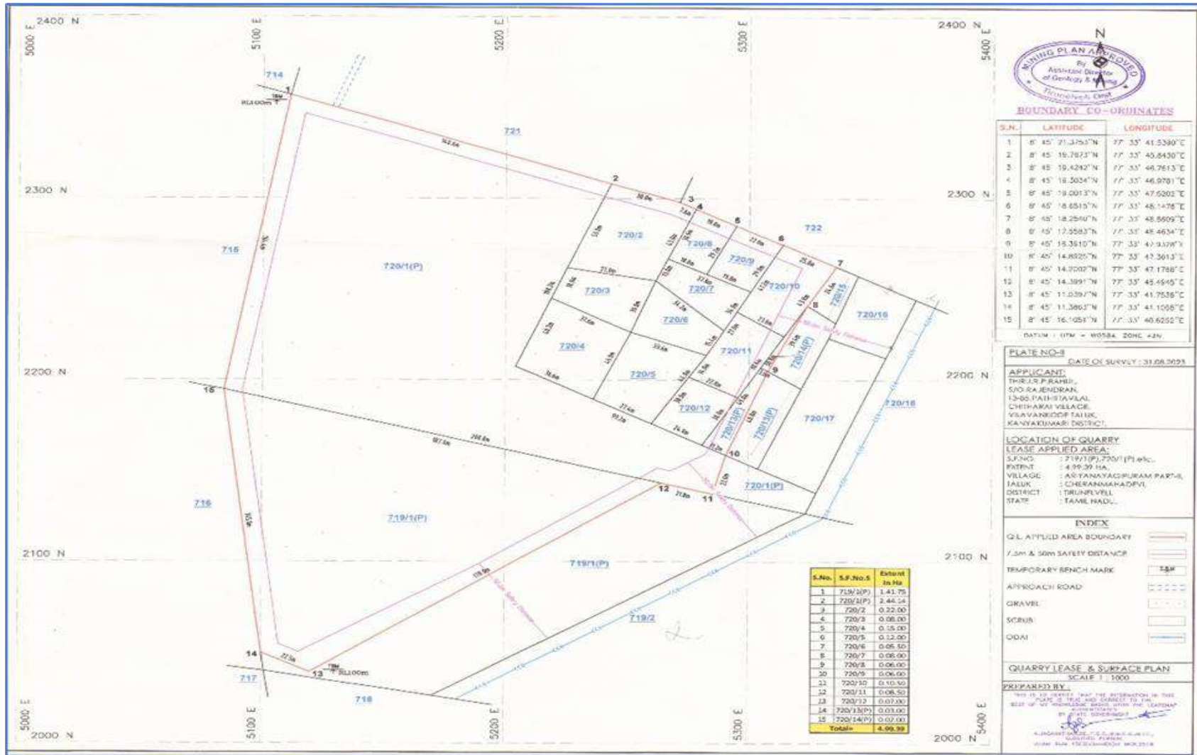
FIGURE 3: QUARRY LEASE PLAN / SURFACE PLAN
