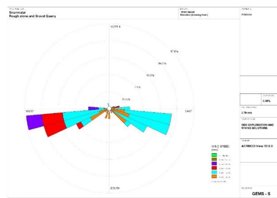
FIGURE – 6: WIND ROSE DIAGRAM
