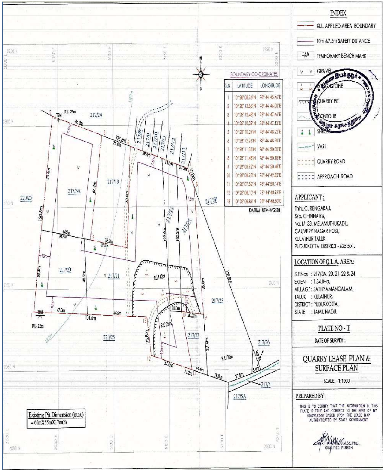
FIGURE – 4: QUARRY LEASE PLAN & SURFACE PLAN
