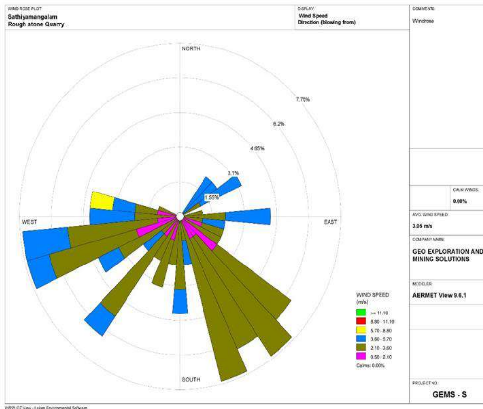
FIGURE – 6: WIND ROSE DIAGRAM
