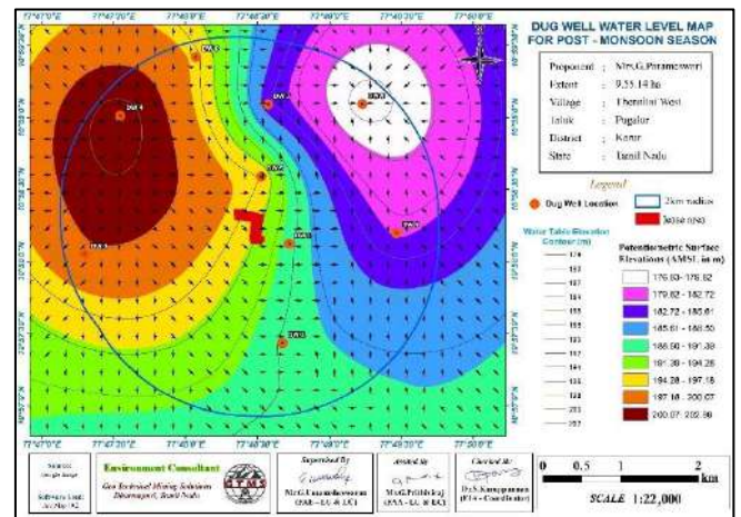
Figure 3.2 Dug well Static Groundwater Elevation Map Showing Direction of Groundwater Flow During Post-Monsoon Season
