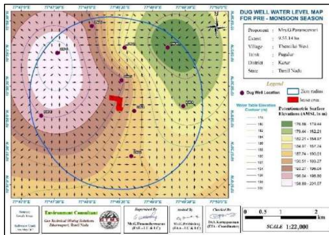
Figure 3.1 Dug well Static Groundwater Elevation Map Showing Direction of Groundwater Flow During Pre-Monsoon Season
