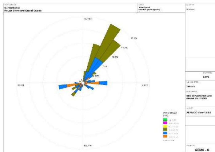
FIGURE – 6: WIND ROSE DIAGRAM
