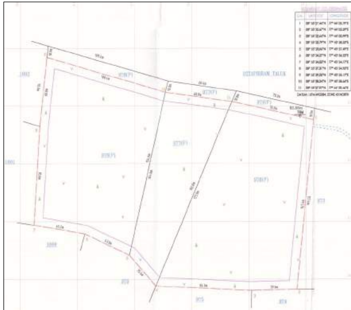
FIGURE 3: QUARRY LEASE PLAN / SURFACE PLAN
