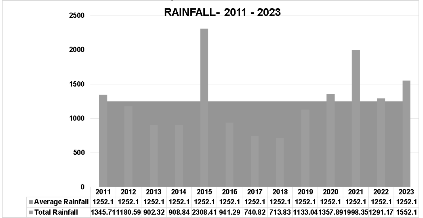
Figure 3.5: Total Rainfall
