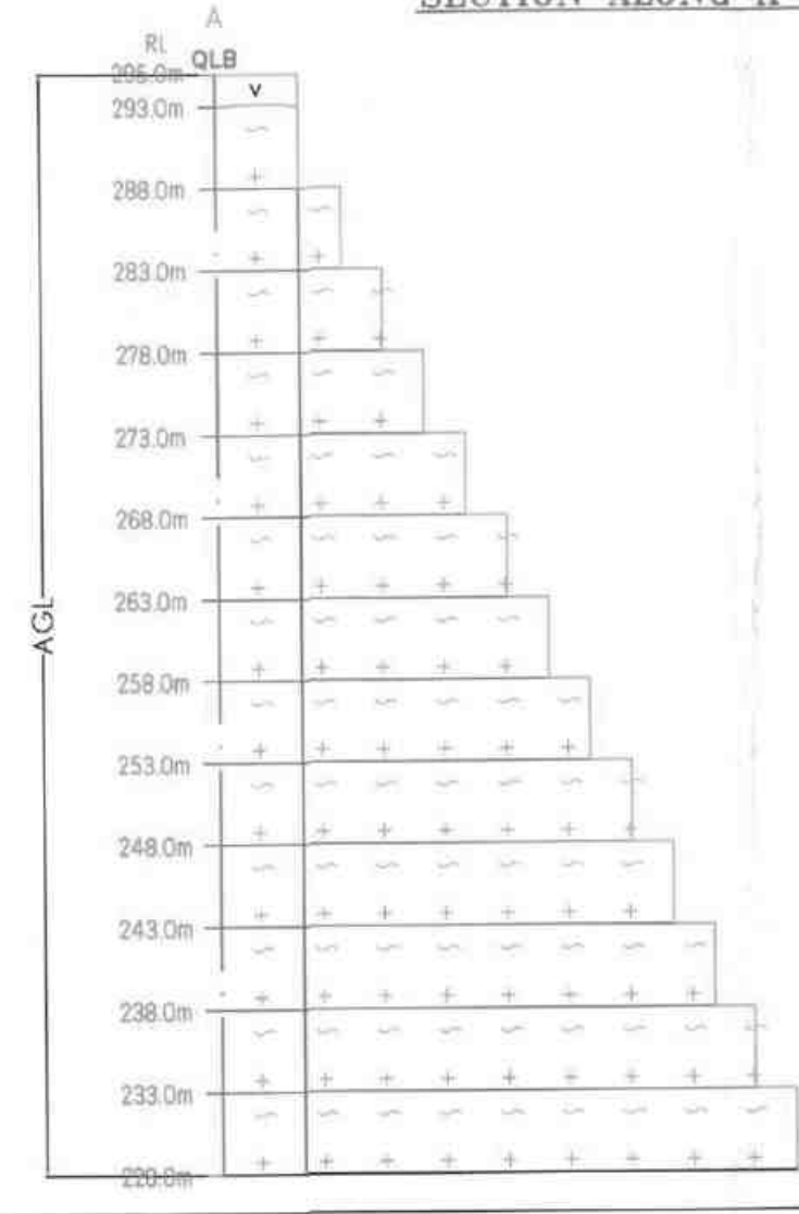
SECTION ALONG A-B
