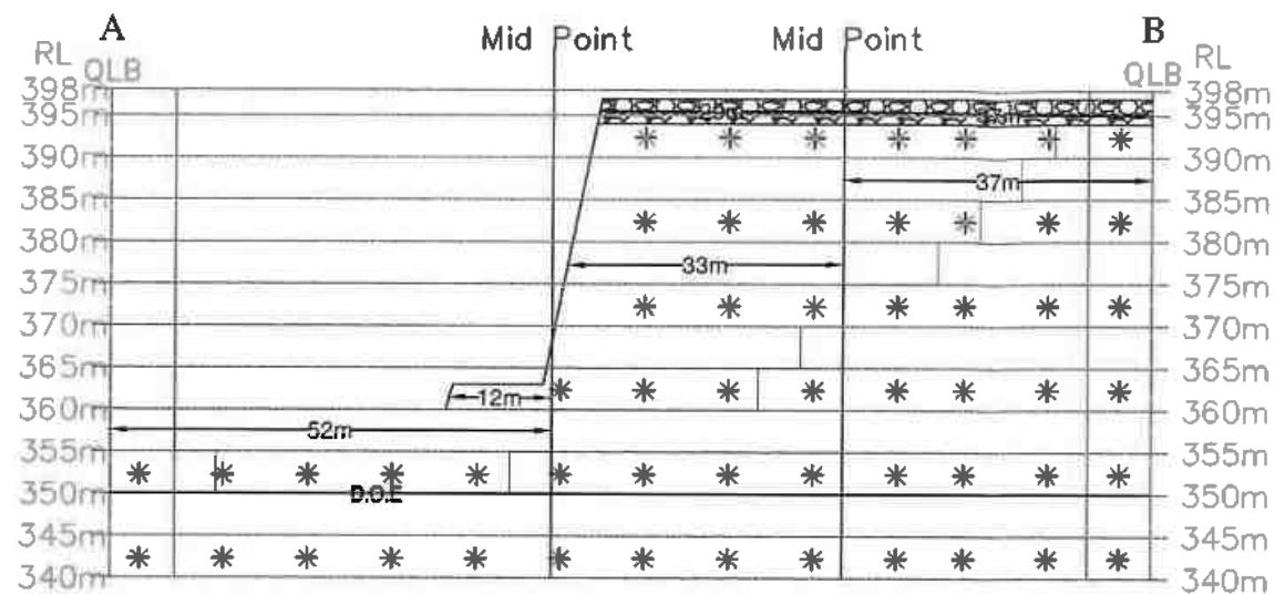
SECTION ALONG A-B
