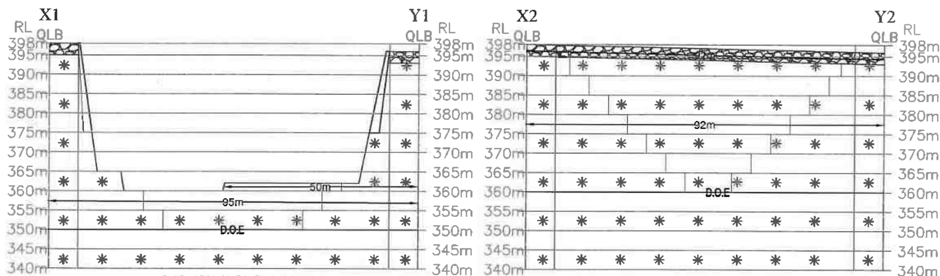
SECTION ALONG X2-Y2
