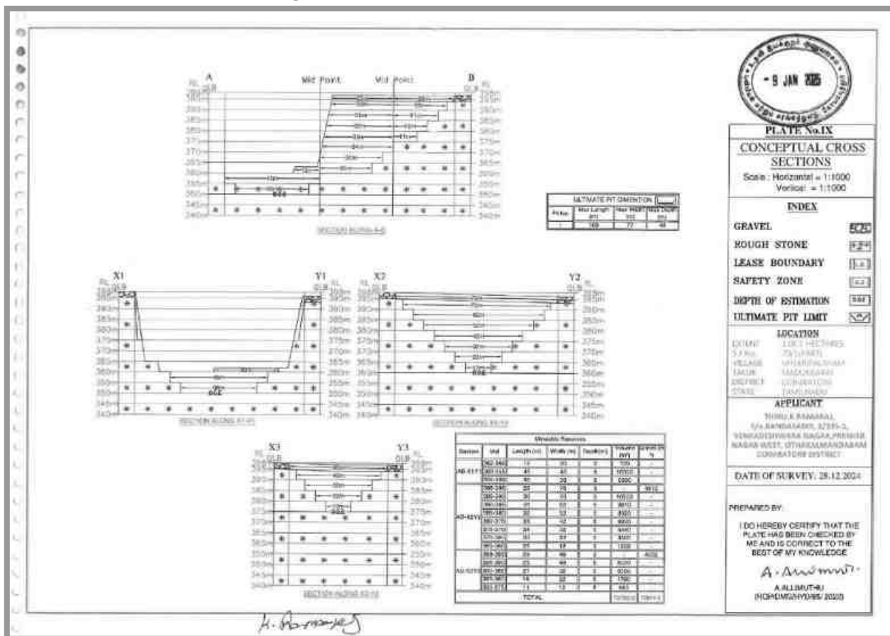
Figure 2.13: Conceptual Cross Section
