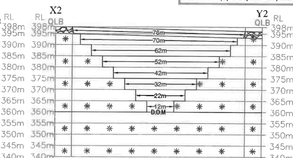
SECTION ALONG X2-Y2
