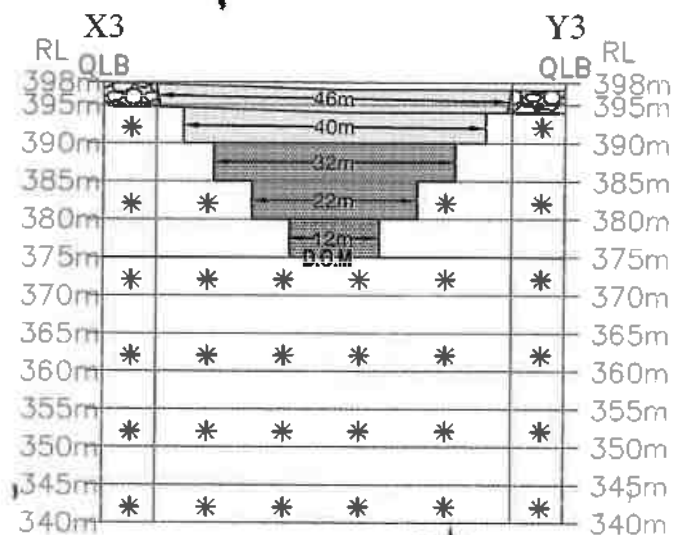
SECTION ALONG X3-Y3
