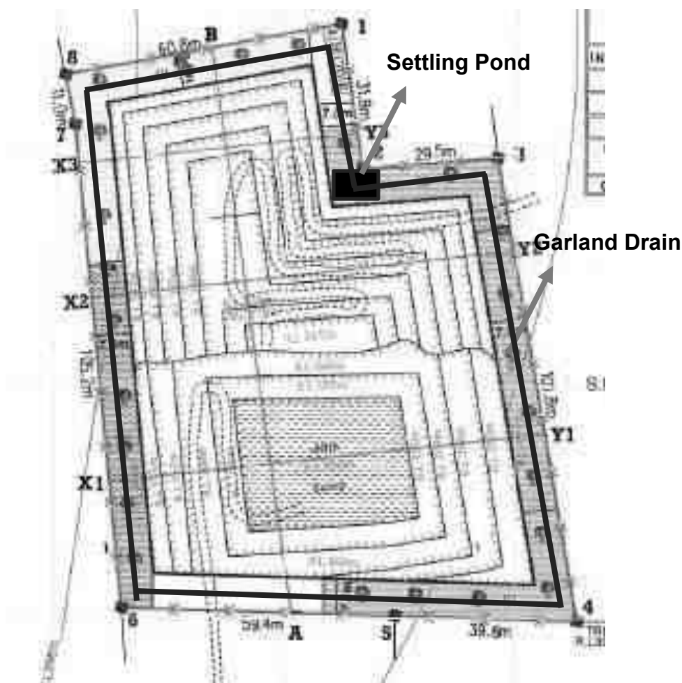
Figure 4.4: Surface Runoff Management Structures
