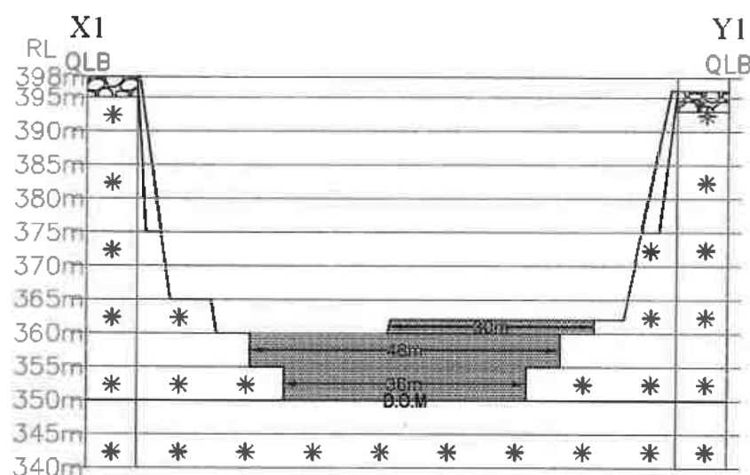
SECTION ALONG X1-Y1
