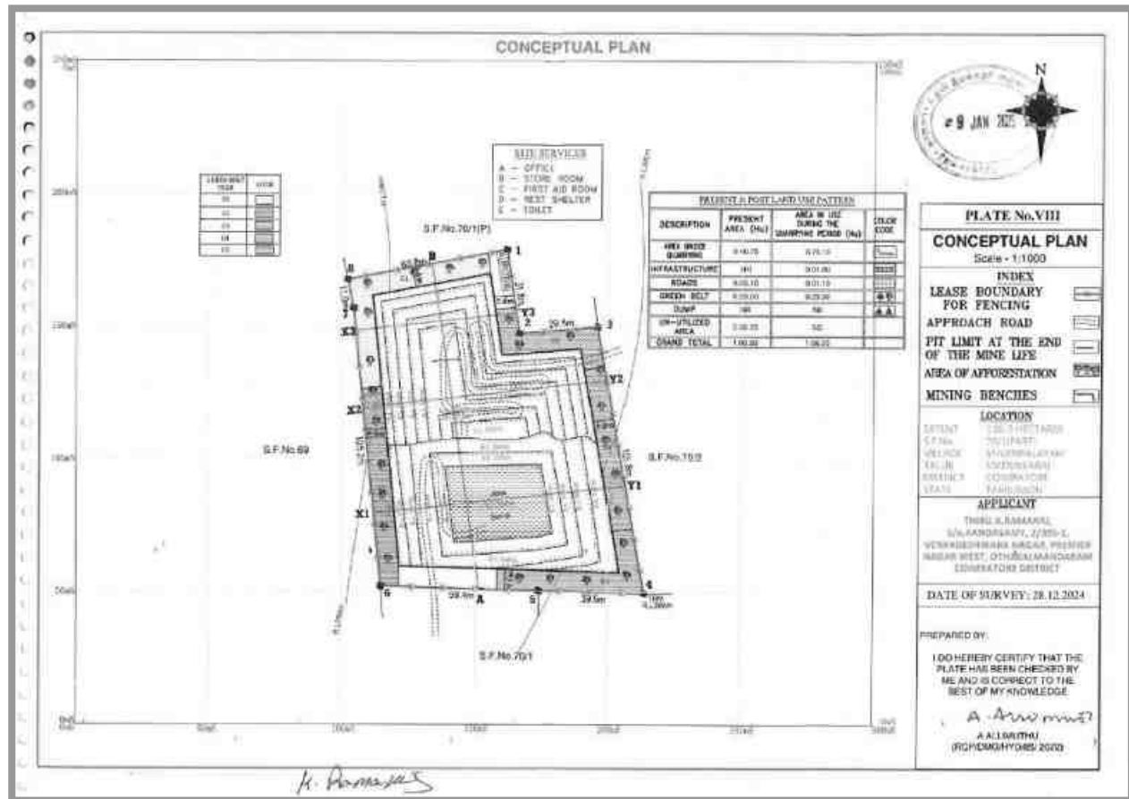
Figure 2.12: Conceptual Plan
