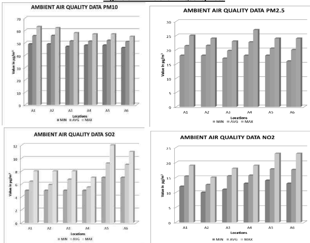
Figure 3.7: Ambient Air Quality Data
