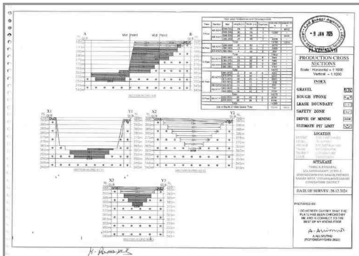
Figure 2.11: Year wise Cross Section
