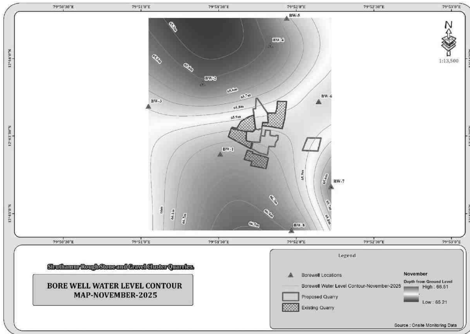
FIGURE 3.10: BOREWELL CONTOUR MAP – NOVEMBER 2025
