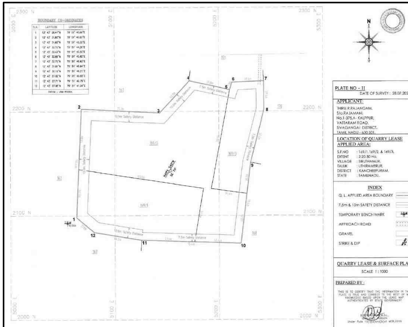
FIGURE 2.7: QUARRY LEASE PLAN / SURFACE PLAN- P1
