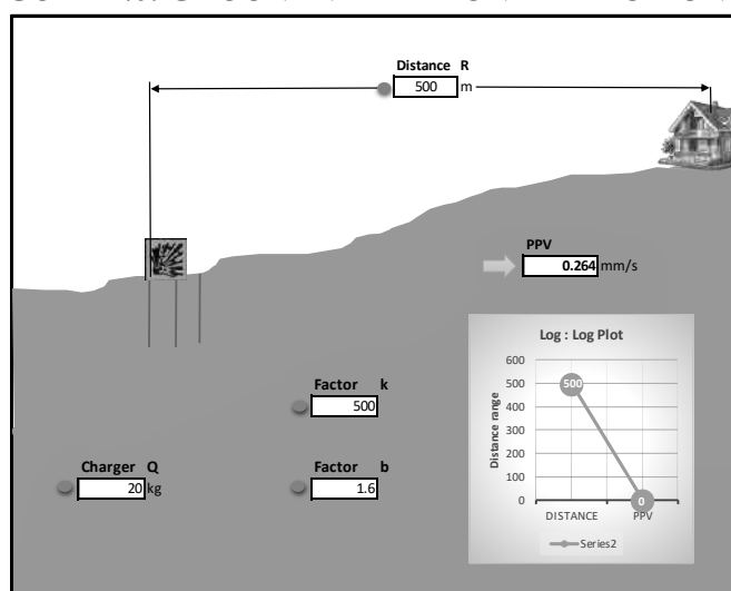
FIGURE 4.6: GROUND VIBRATION PREDICTION- P2
