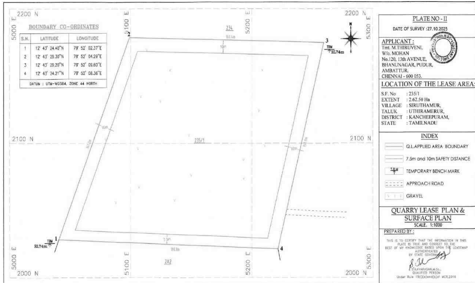
FIGURE 2.8A: QUARRY LEASE PLAN / SURFACE PLAN- P3
