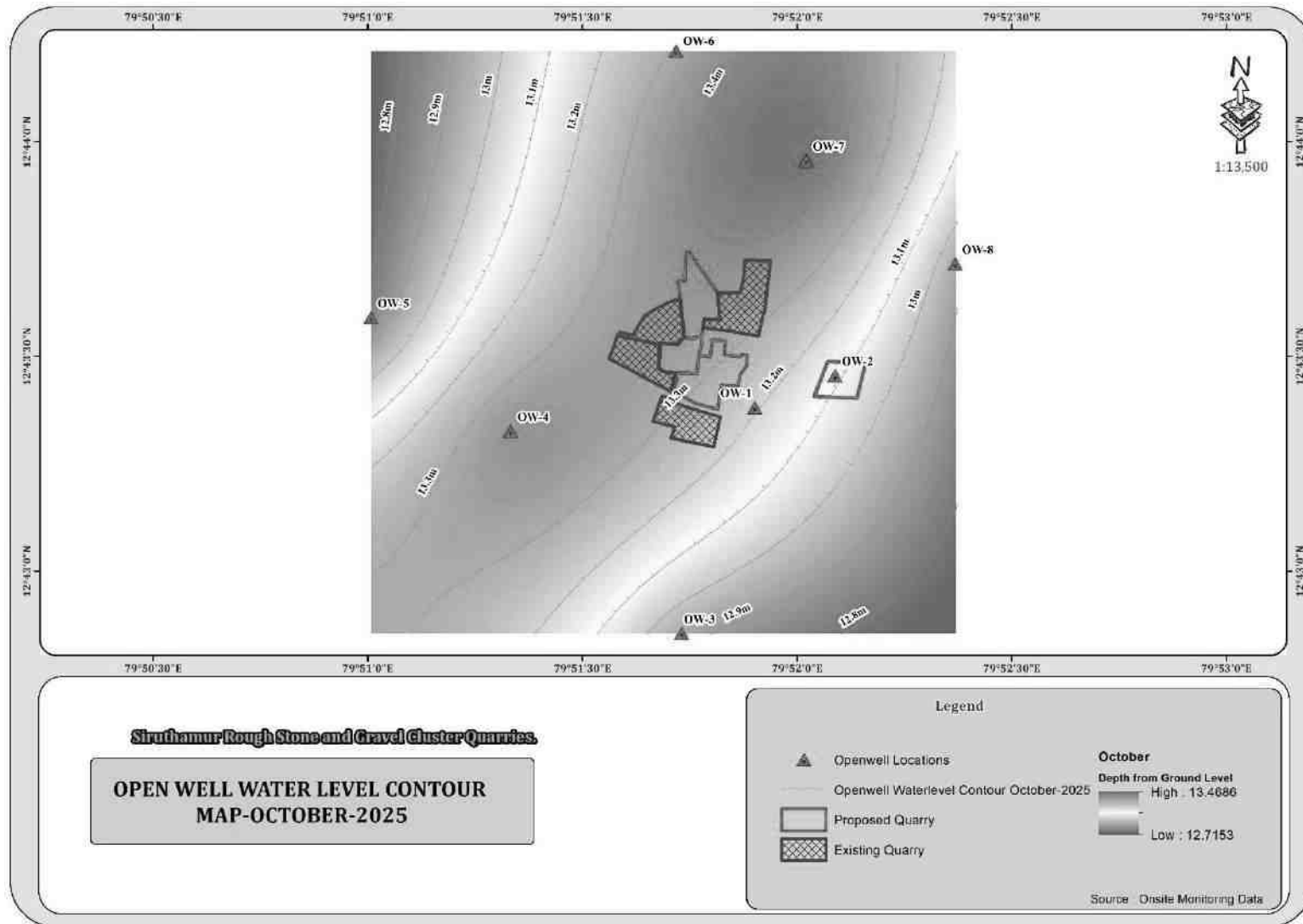
FIGURE 3.6: OPEN WELL CONTOUR MAP – OCTOBER 2025
