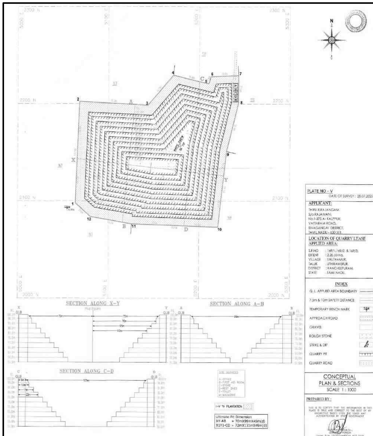
FIGURE 2.17: CLOSURE PLAN AND SECTIONS- P1
