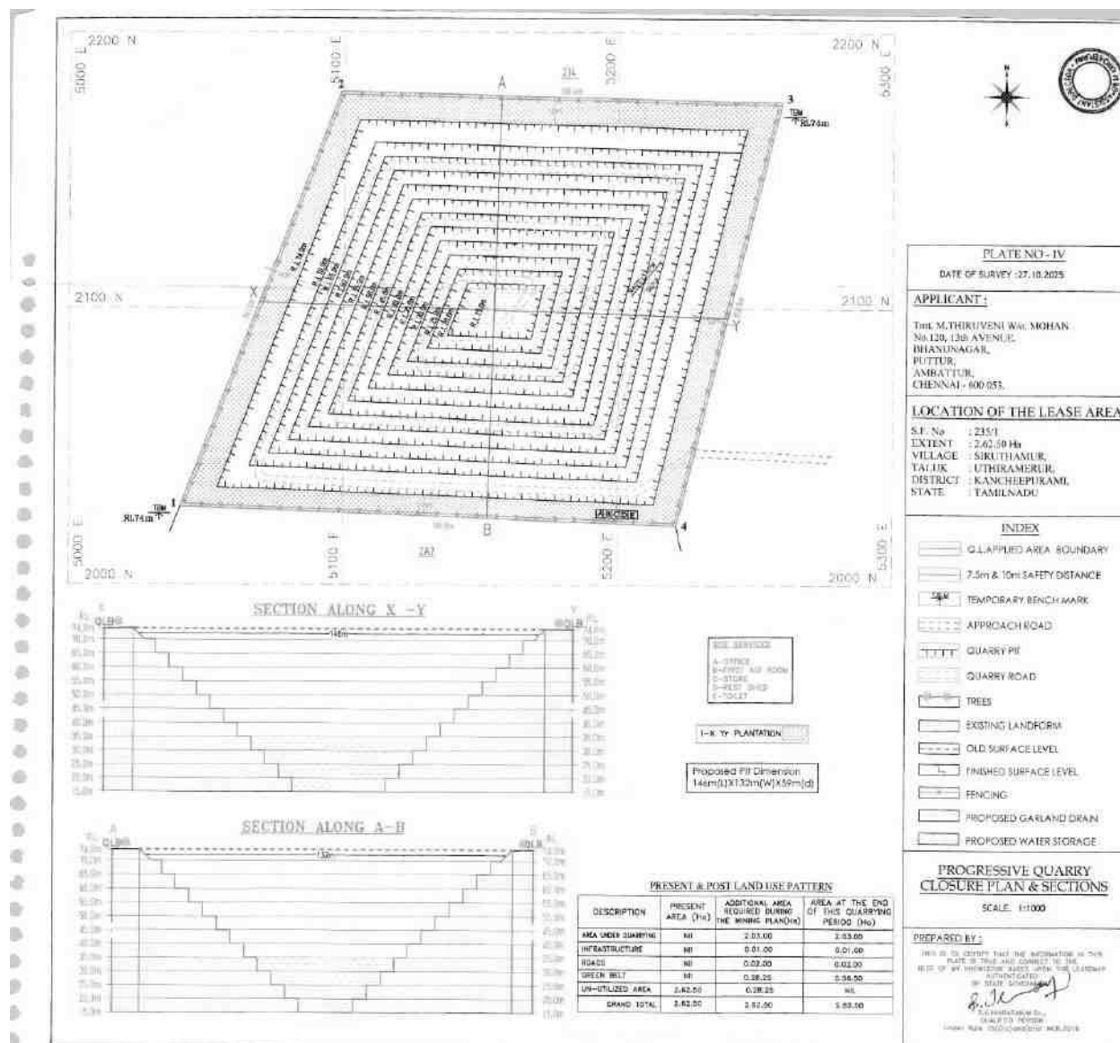
FIGURE 2.18A: CLOSURE PLAN AND SECTIONS- P3
