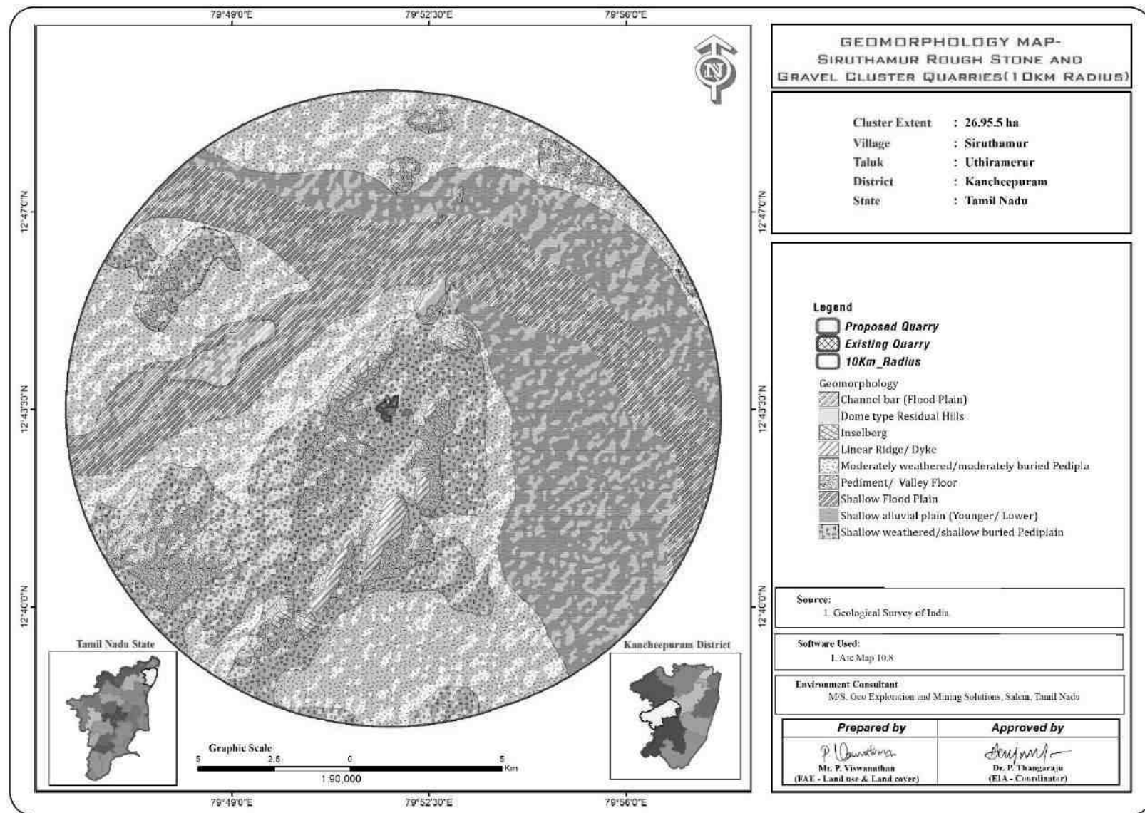
FIGURE 2.14: GEOMORPHOLOGY MAP
