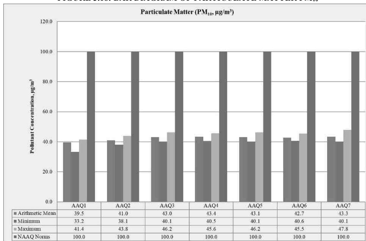
FIGURE 3.18: BAR DIAGRAM OF PARTICULATE MATTER PM 10
