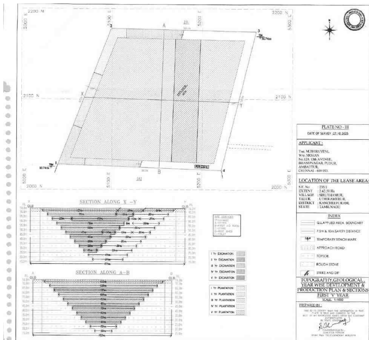
FIGURE 2.16A: TOPOGRAPHY, GEOLOGICAL, YEAR-WISE DEVELOPMENT PRODUCTION PLAN AND SECTIONS FOR FIRST FIVE YEAR- P3
