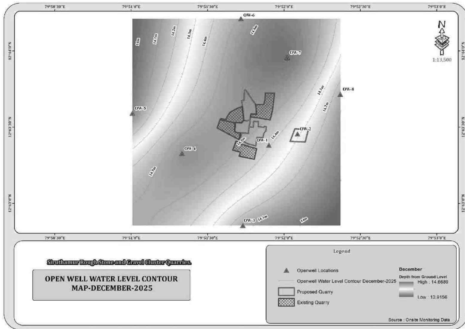
FIGURE 3.8: OPEN WELL CONTOUR MAP – DECEMBER 2025
