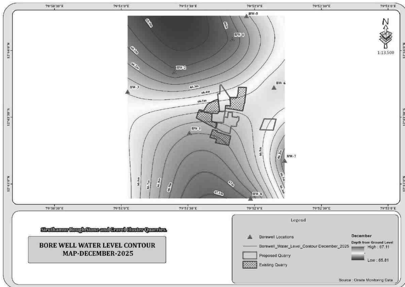
FIGURE 3.11: BOREWELL CONTOUR MAP – DECEMBER 2025
