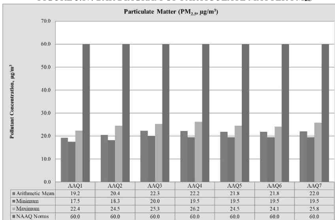
FIGURE 3.17: BAR DIAGRAM OF PARTICULATE MATTER PM 2.5
