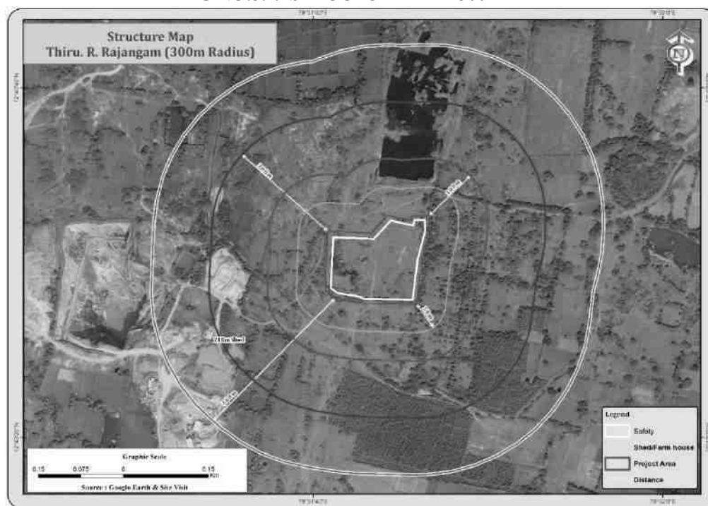
FIG NO:3.29 STRUCTURE MAP 300M – P1
