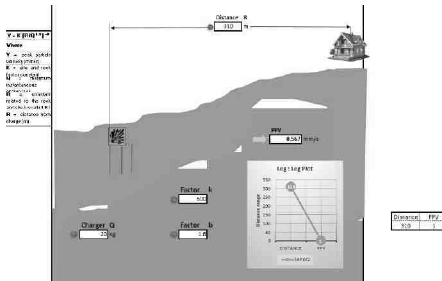
FIGURE 4.6A: GROUND VIBRATION PREDICTION- P3
