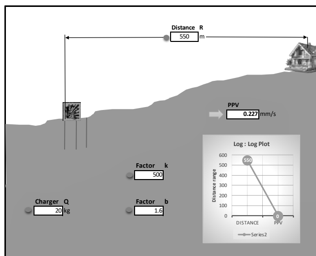
FIGURE 4.6: GROUND VIBRATION PREDICTION- P1
