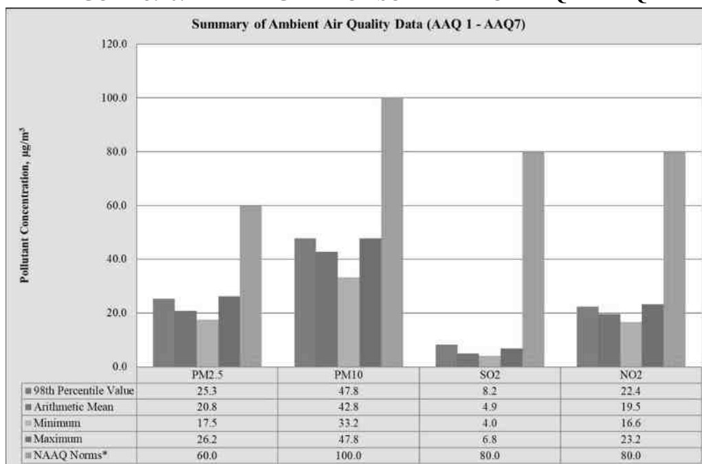
FIGURE 3.16: BAR DIAGRAM OF SUMMARY OF AAQ 1 – AAQ7
