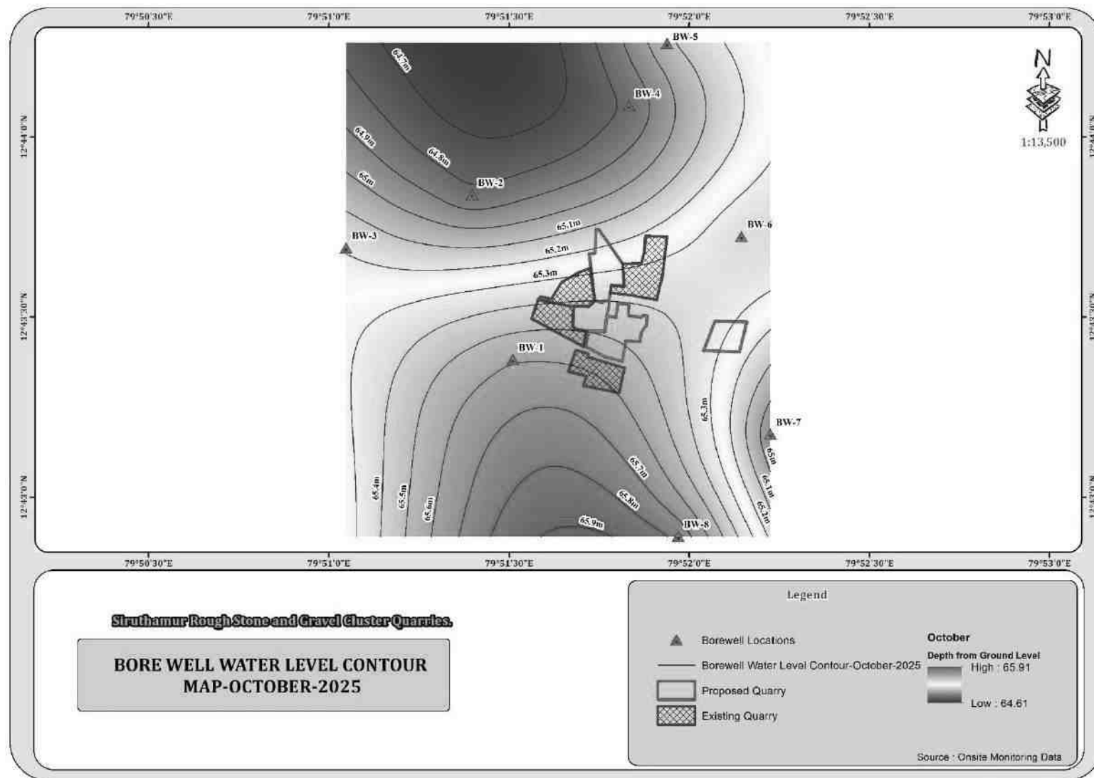
FIGURE 3.9: BOREWELL CONTOUR MAP – OCTOBER 2025
