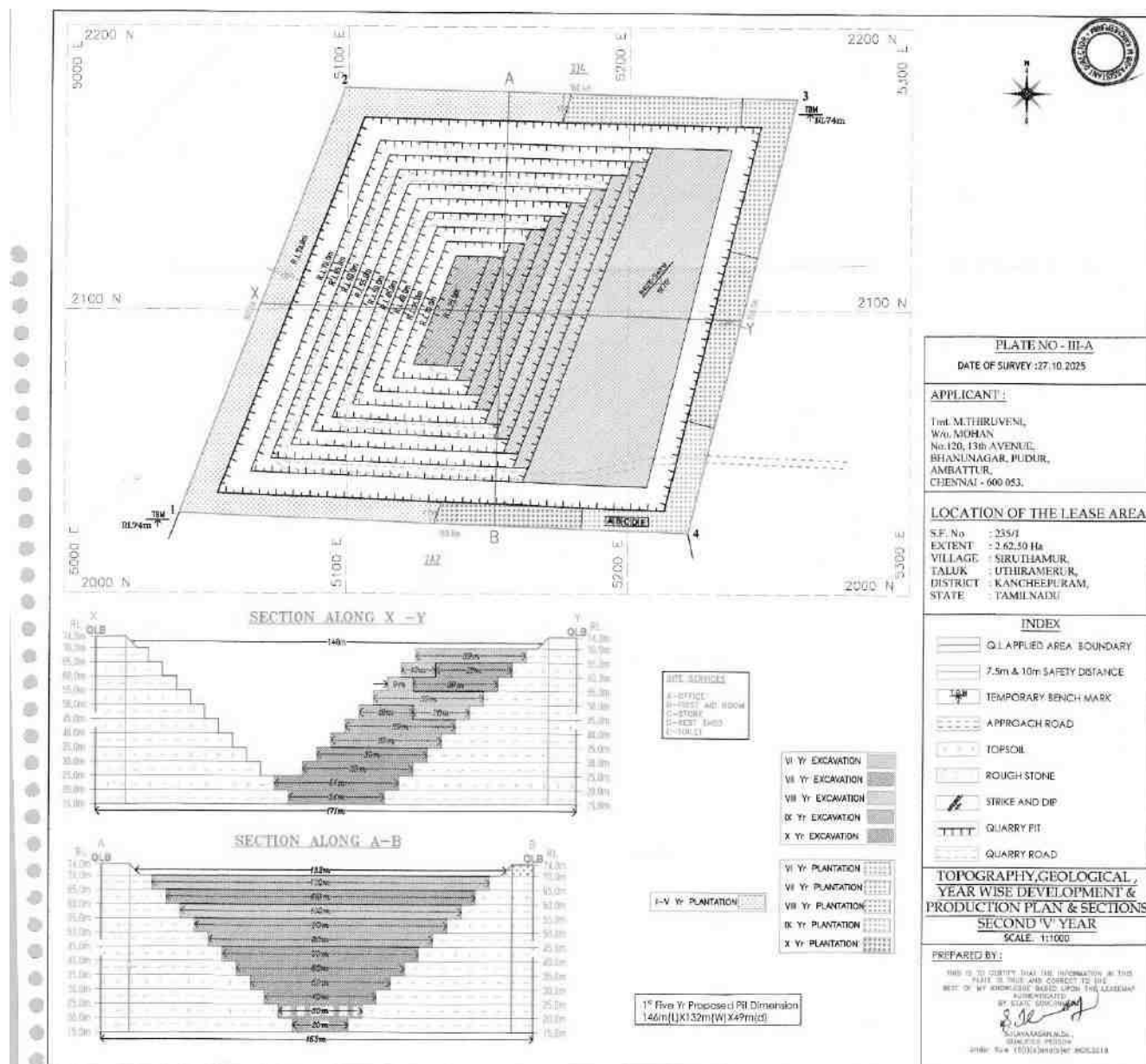
FIGURE 2.16A: TOPOGRAPHY, GEOLOGICAL, YEAR-WISE DEVELOPMENT PRODUCTION PLAN AND SECTIONS FOR SECOND FIVE YEAR- P3
