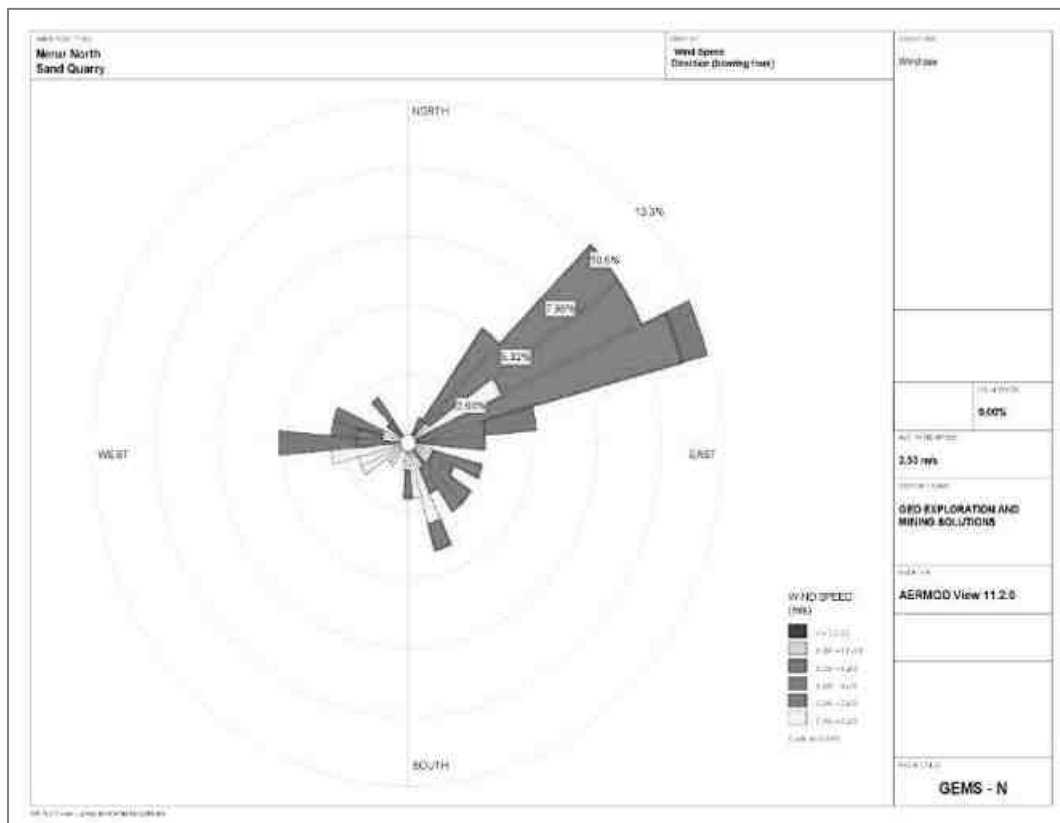
FIGURE 3.9: WINDROSE DIAGRAM
