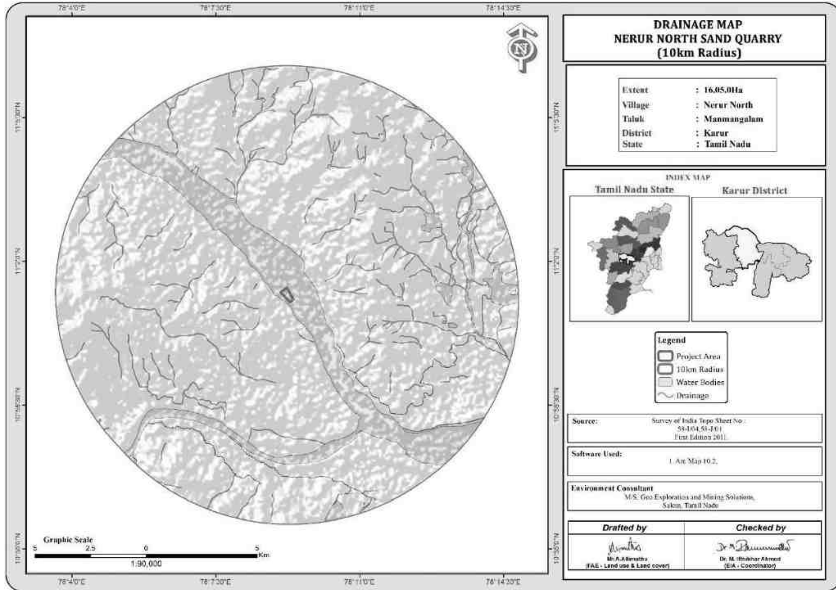
Figure 3.8: Drainage map of the study area - 10km radius
