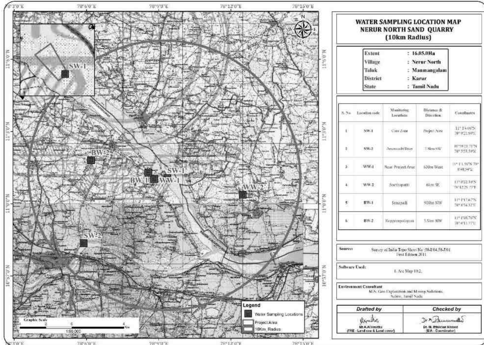
Figure 3.6: Water quality monitoring stations around 10km radius
