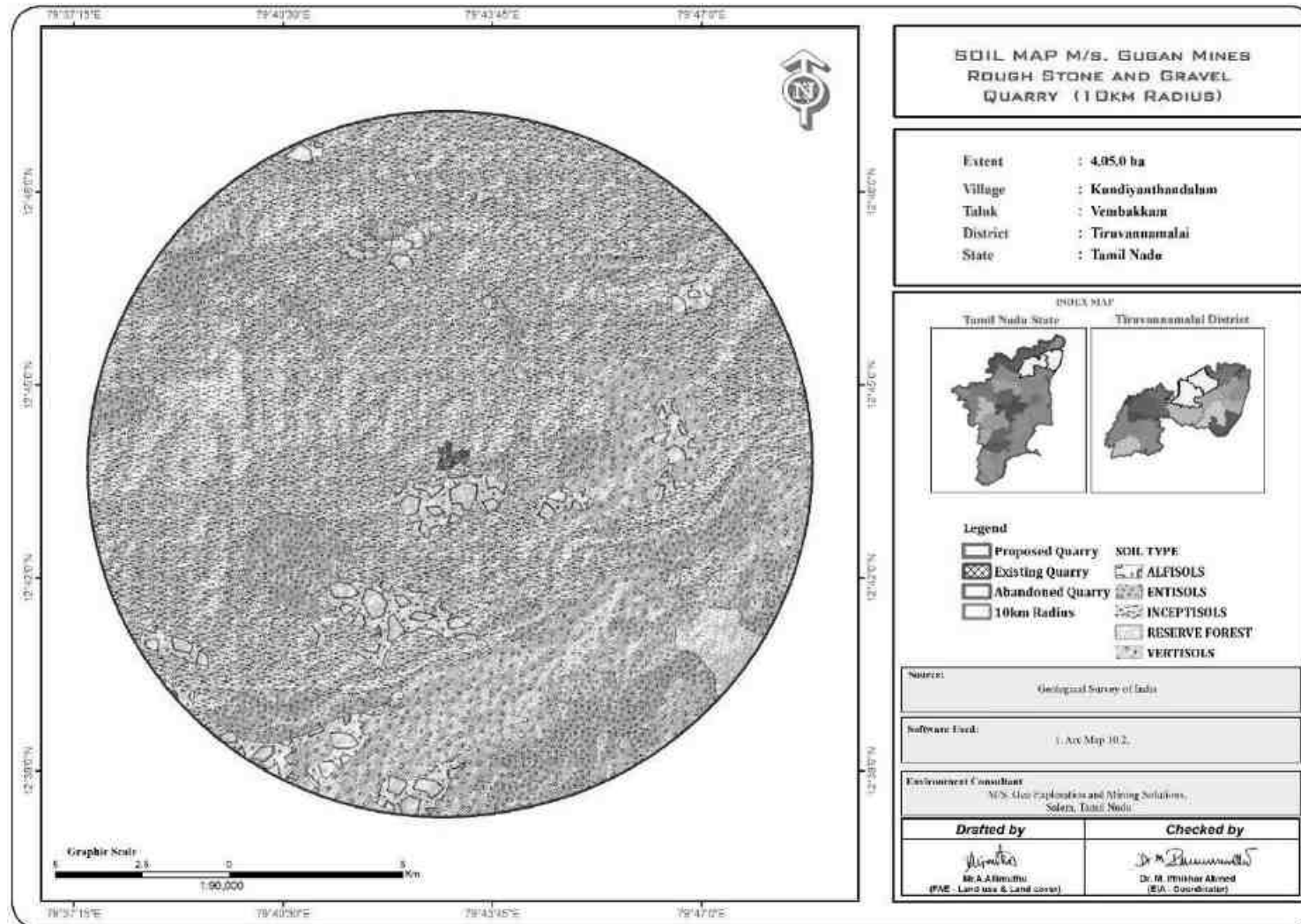
FIGURE 3.6: SOIL MAP
