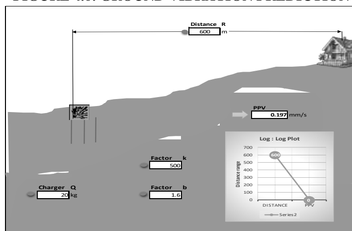
FIGURE 4.6: GROUND VIBRATION PREDICTION
