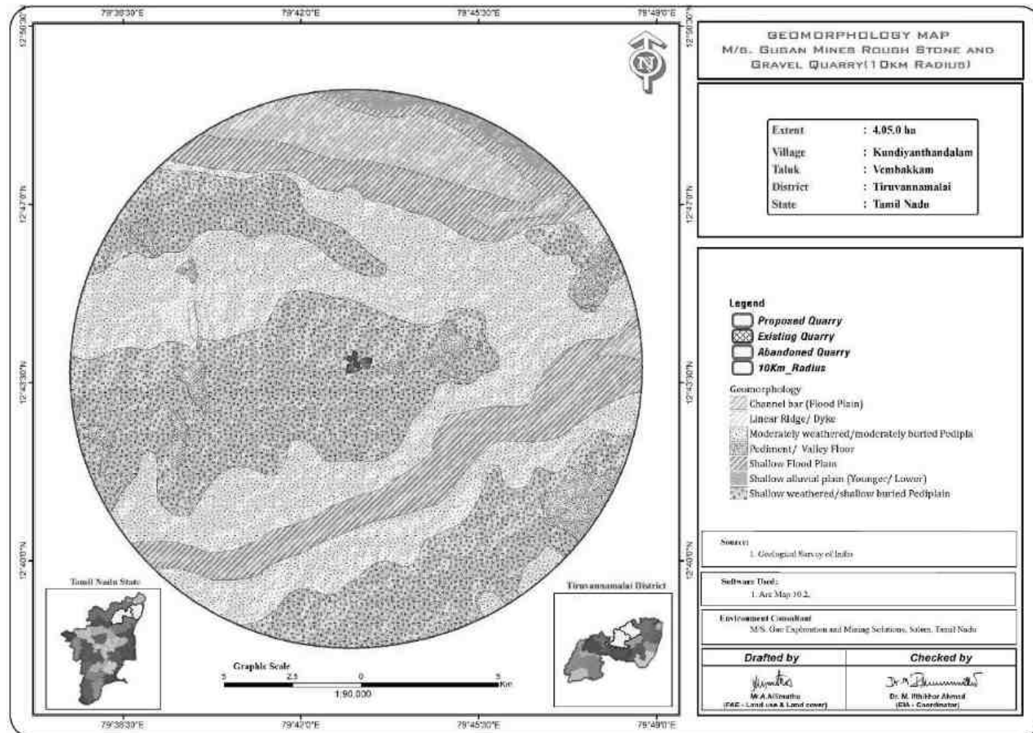
FIGURE 2.11: GEOMORPHOLOGY MAP
