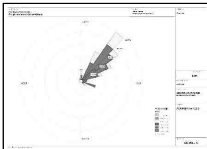
FIGURE 3.13: WINDROSE DIAGRAM
